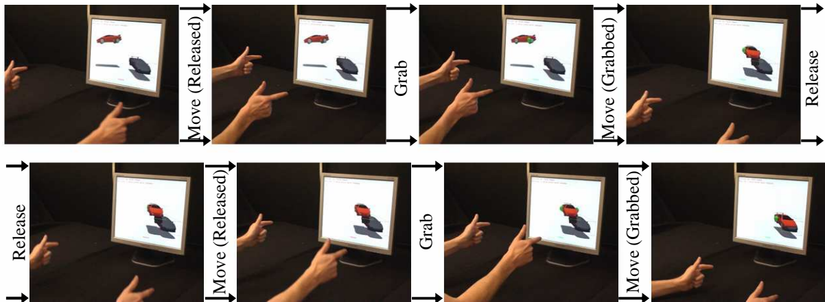
Figure 1: Image sequence of our demo system. Based on our bimanual symmetric interaction technique a virtual object (red car) can be grabbed (move hands together), manipulated (as if gripped between hands) and released (move hands apart).
