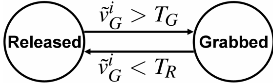
Figure 3: State machine illustrating how an object can be grabbed and released. Thresholds T_G and T_R are applied to the modified signed grabbing velocity \tilde{v}_G^i .
