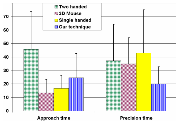
Figure 6: Completion times (in seconds) with standard deviations (error bars).
